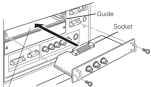
Plug Figure shows Dual-SDI terminal.
